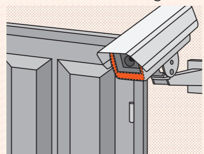
Paste the heater around the lens, to prevent the lens from moving.
